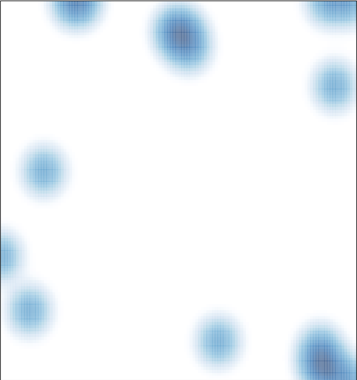
# features = 16 , max = 1
